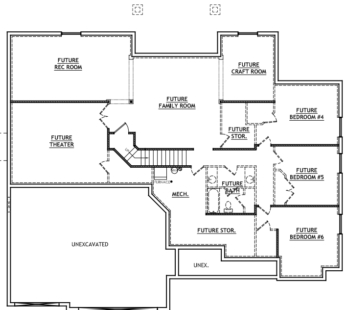
UNFINISHED BASEMENT (OPT. 9' WALLS)
